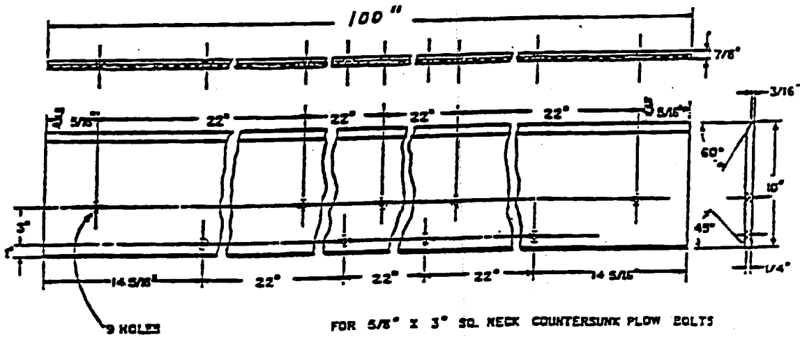
LOADER BUCKET CUTTING EDGE
