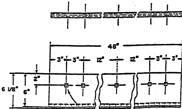
SNOW PLOW CUTTING EDGE
